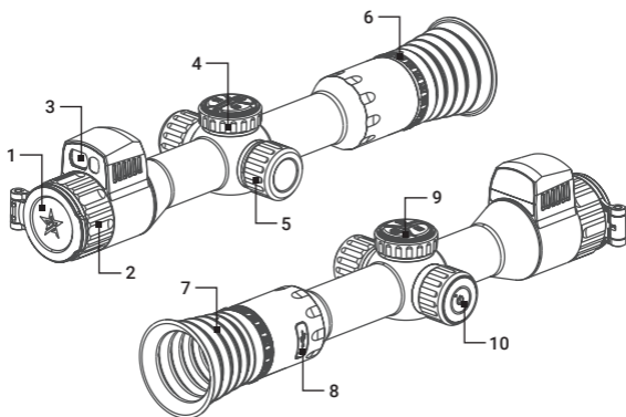
FIGURE 1-1. MAIN PARTS
