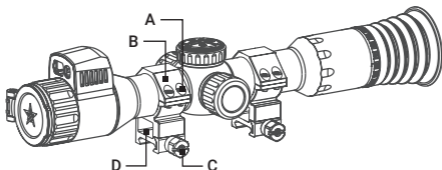
FIGURE 2-5. INSTALLATION WITH SCOPE RINGS
