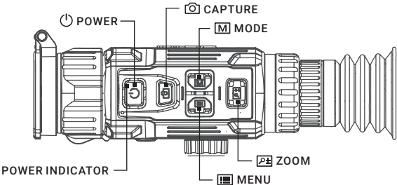
FIGURE 2-2. CONTROL BUTTONS
