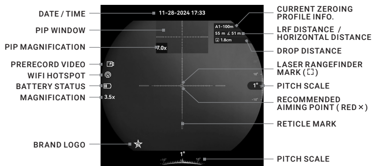
FIGURE 2-3. ON-SCREEN DISPLAY
