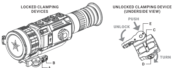
FIGURE 2-5. MOUNT
